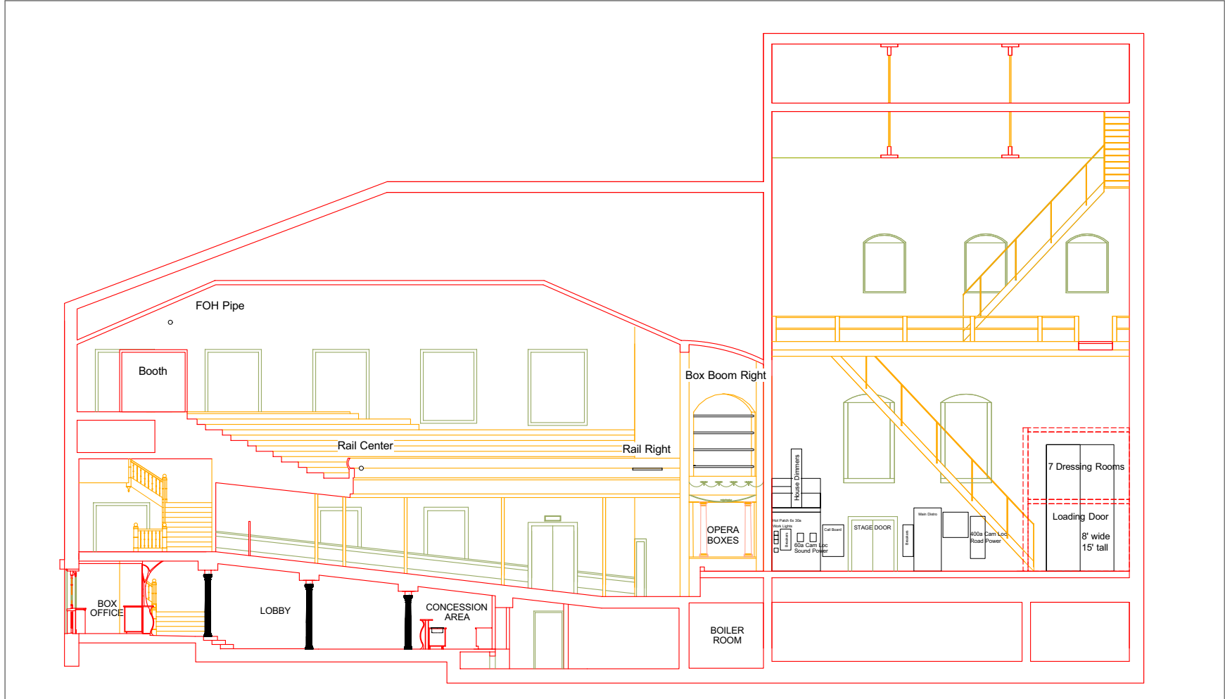
Center Line Section Looking Stage Right
